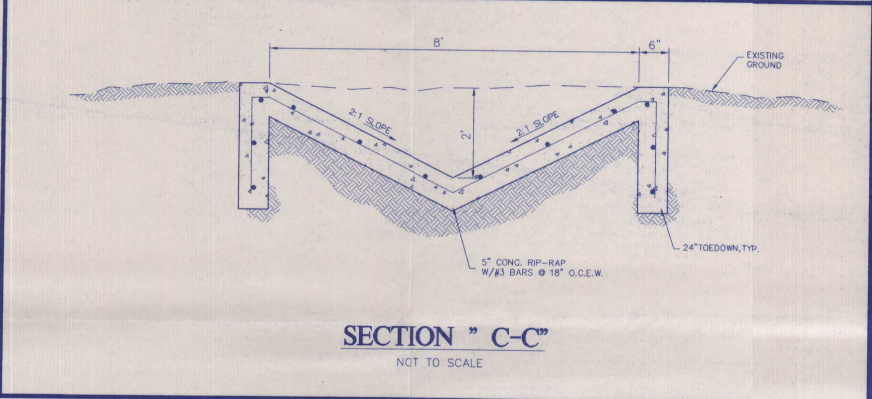
INLET/OVERFLOW STRUCTURE NOT TO SCALE
