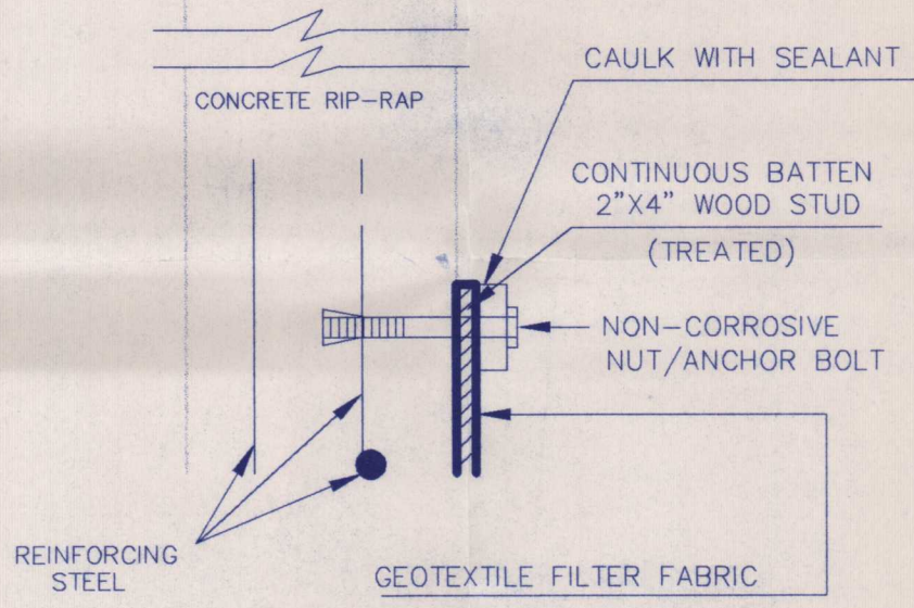
GEOTEXTILE FILTER FABRIC ANCHORING DETAIL N.T.S.
